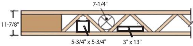
Spans up to 22'00"
